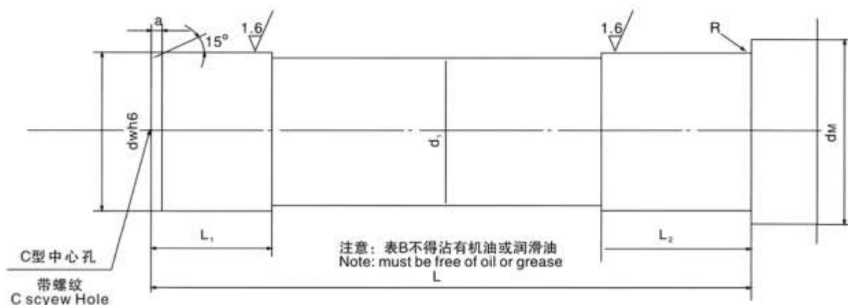
图10胀盘联接的轴 Sheet10: shaft for shrind disks
