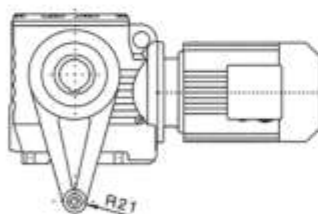
YFS..S67 ★
