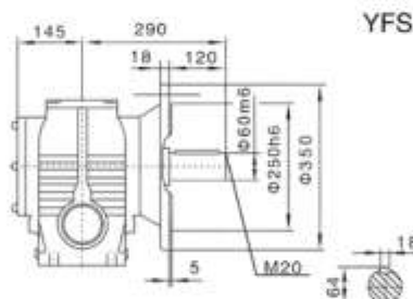
YFSF87
