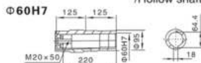
YFSA87/YFSAZ87/YFSAF87/空心轴 /Hollow shaft
