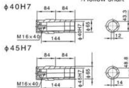
YFSA67/YFAZ67/YFSAF67/空心轴/Hollow shaft
