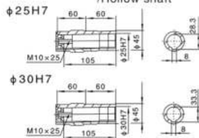
YFSA47/YFSAZ47/YFSAF47/空心轴 /Hollow shaft
