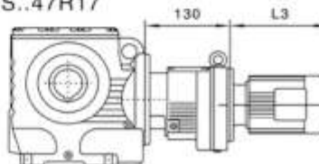
YFS..47R17
