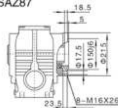
YFSAZ87
