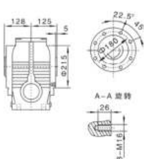
YFSAZ87
