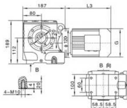
YFSA57
