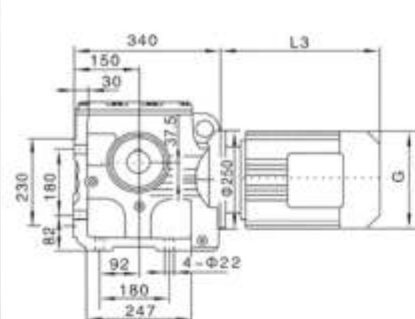
YFS87
