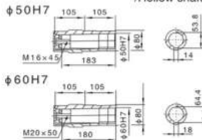
YFSA77/YFSAZ77/YFSAF77/空心轴/Hollow shaft
