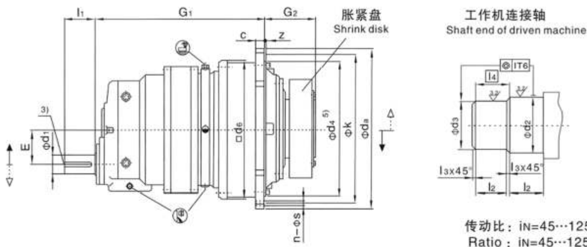
型号YFP2SAZ/规格9...36/Type YFP2SAZ/Sizes 9...36
