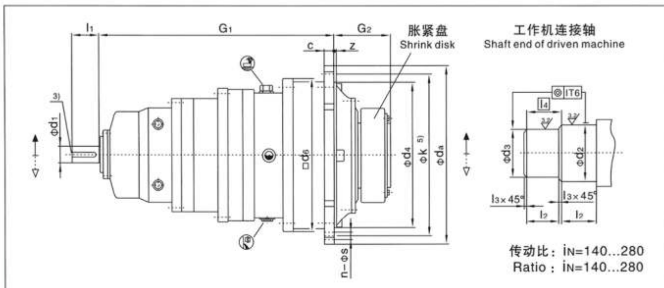
型号YFP3NAZ/规格9...36/TypeYFP3NAZ/Sizes 9...36
